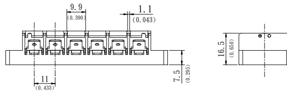
ETBT140X2F000Z #250 Quick connect terminal Pitch=11.0mm
