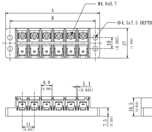
ETBT140X2K000Z #250 Quick connect terminal Pitch=11.0mm
