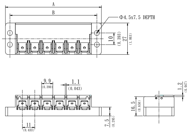
ETBT140X2F000Z #250 Quick connect terminal Pitch=11.0mm
